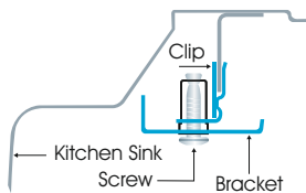
Fit Sink in the Platform
